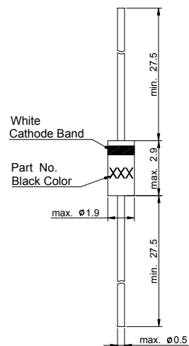
Glass case JEDEC DO-34 Dimensions in mm
